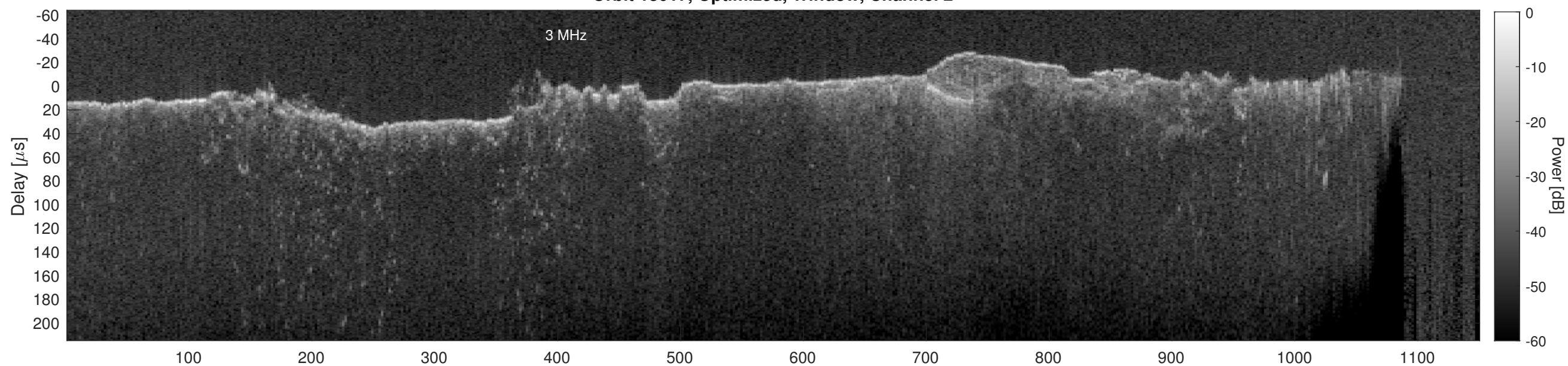
Orbit 13017, Cluttergram
