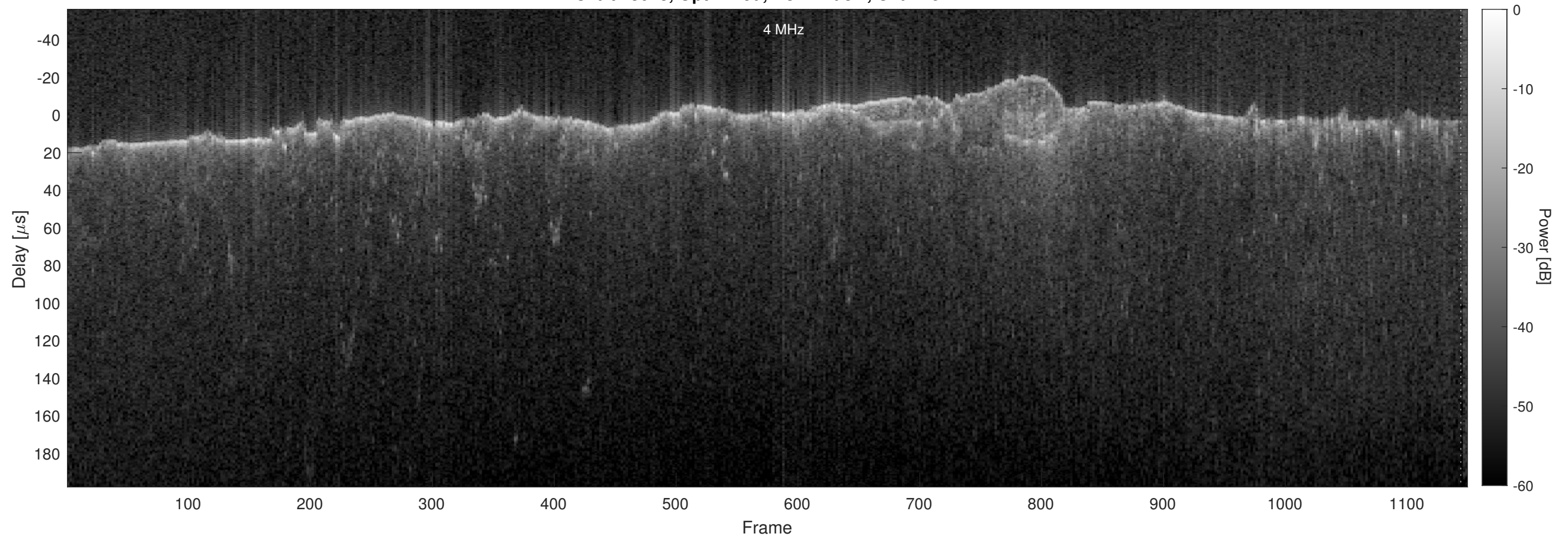
Orbit 13018, Optimized, No Window, Channel 2
