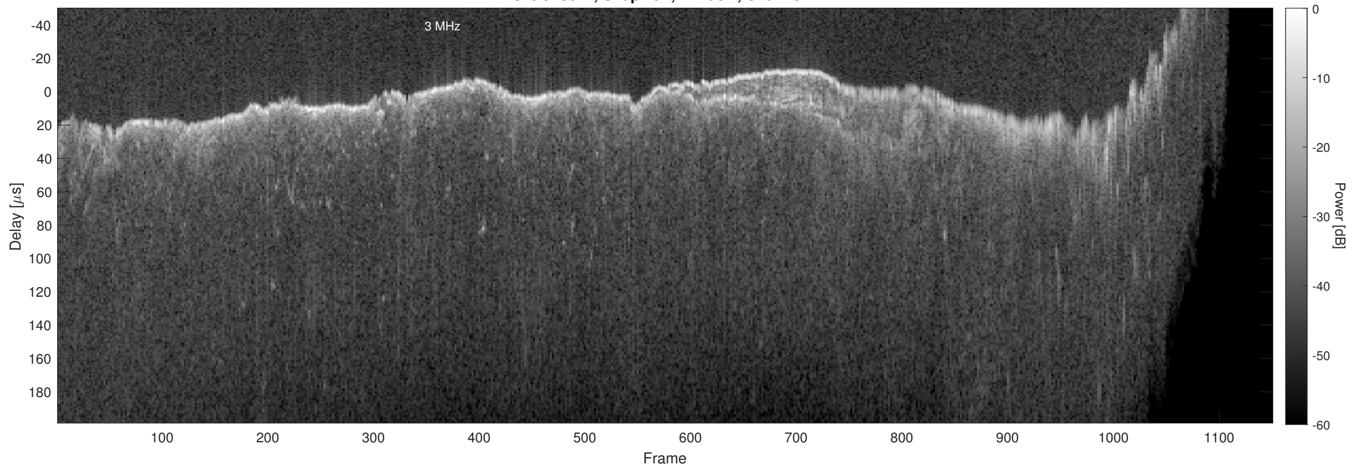
Orbit 13022, Chapman, Window, Channel 2
