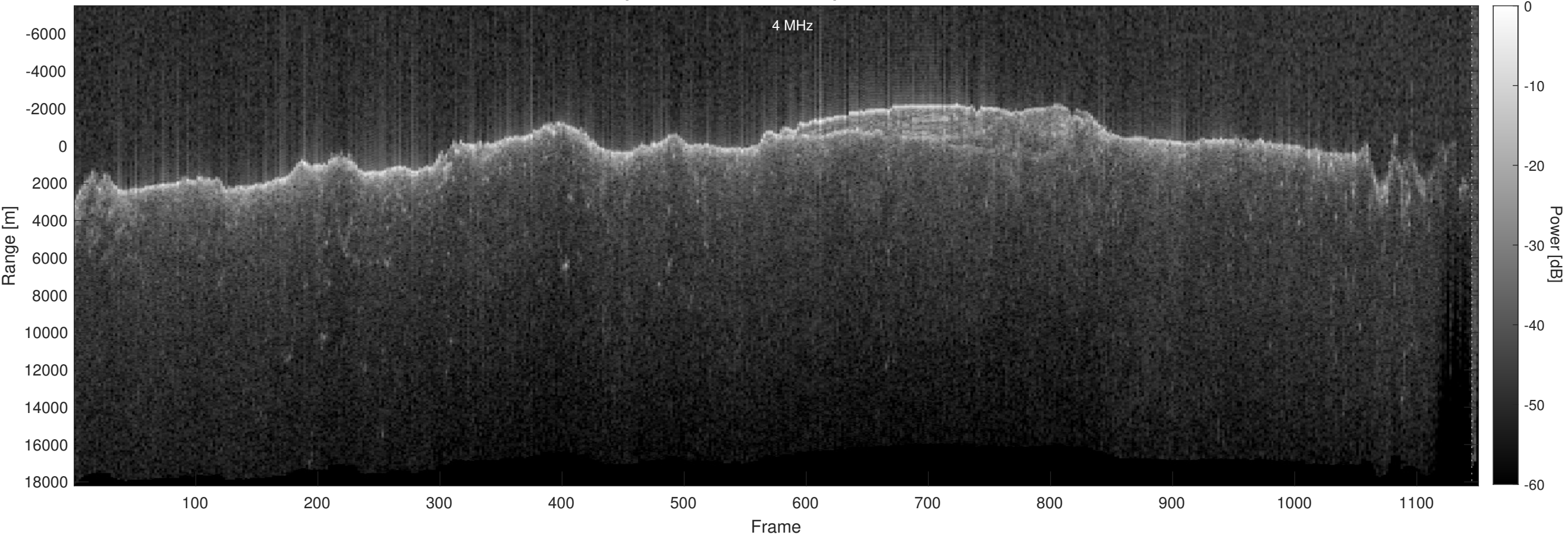
Orbit 13022, Optimized, No Window, Depth-Corrected, Channel 2
