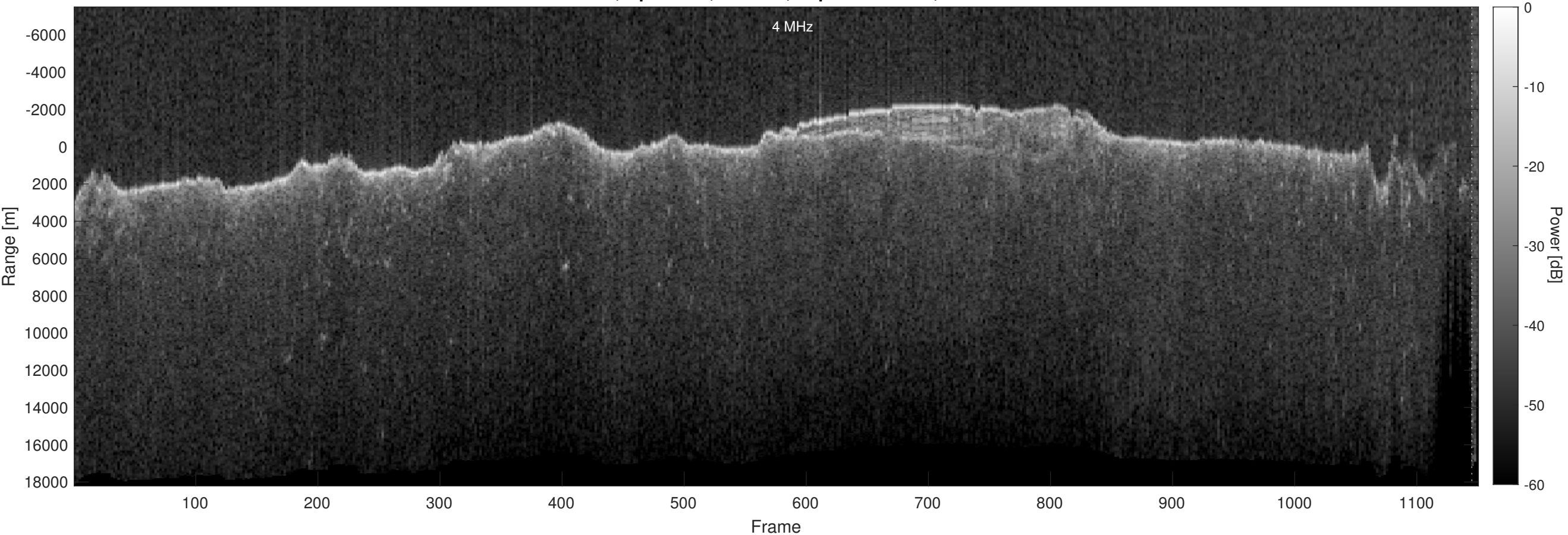
Orbit 13022, Optimized, Window, Depth-Corrected, Channel 2
