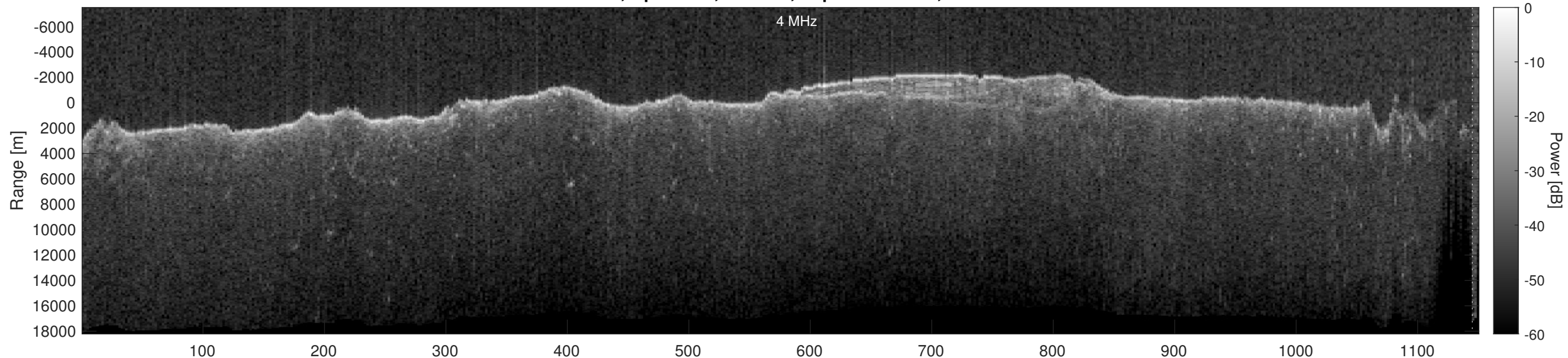
Orbit 13022, Optimized, Window, Depth-Corrected, Channel 2
