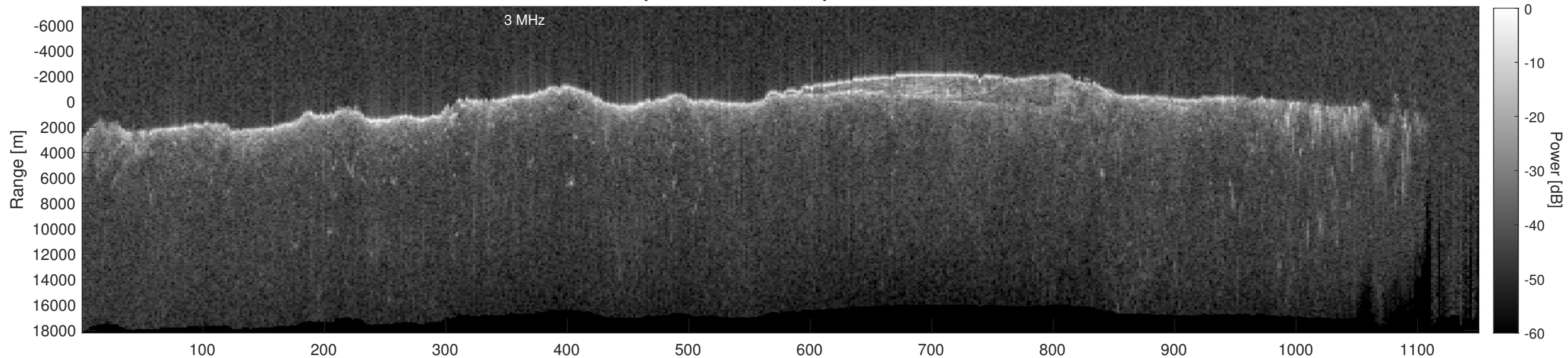
Orbit 13022, Depth-Corrected Cluttergram
