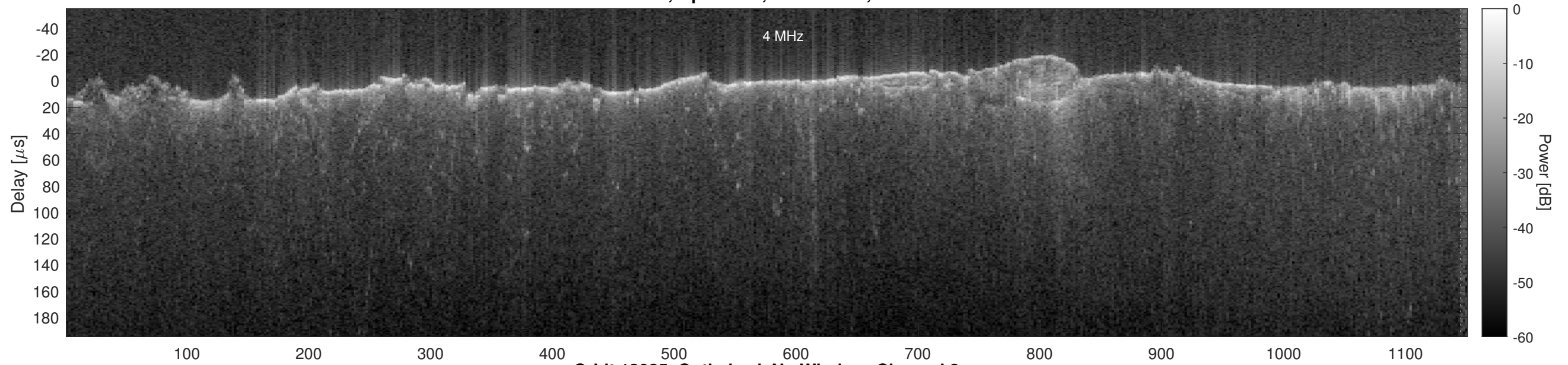
Orbit 13025, Optimized, No Window, Channel 2
