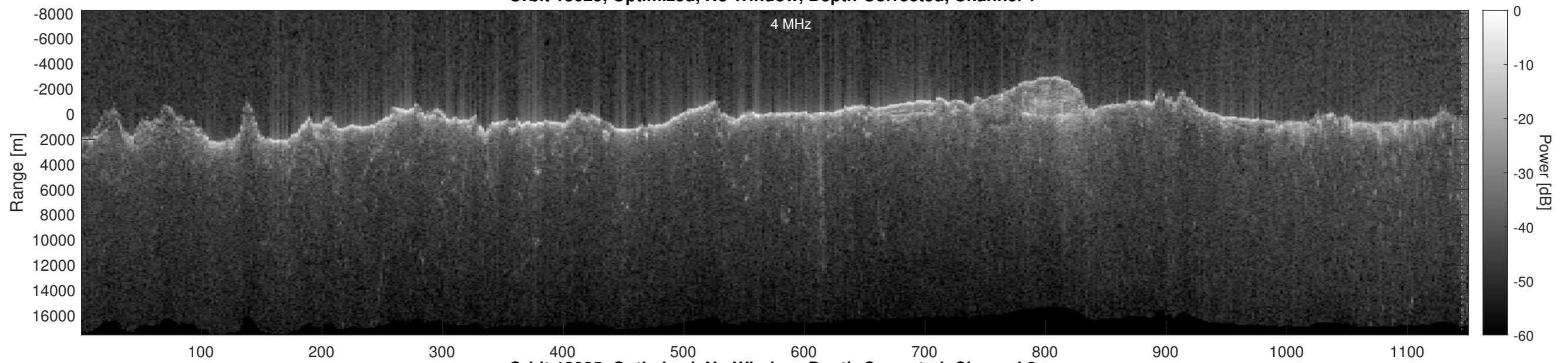
Orbit 13025, Optimized, No Window, Depth-Corrected, Channel 2
