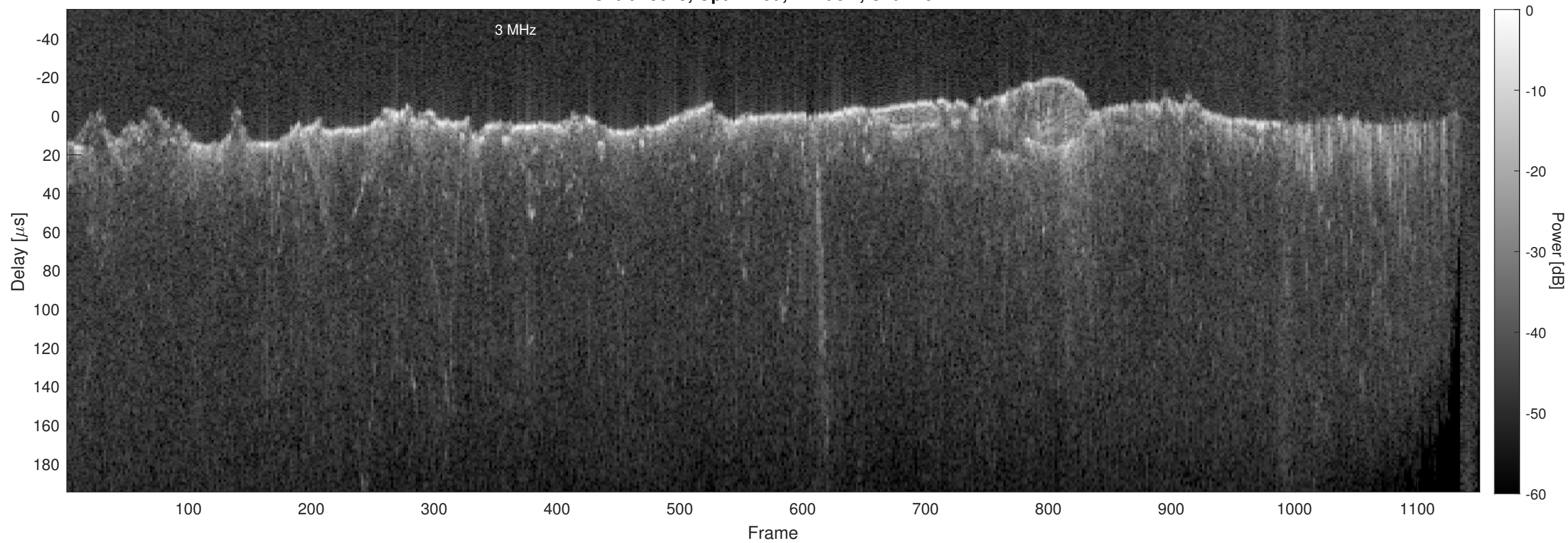
Orbit 13025, Optimized, Window, Channel 2
