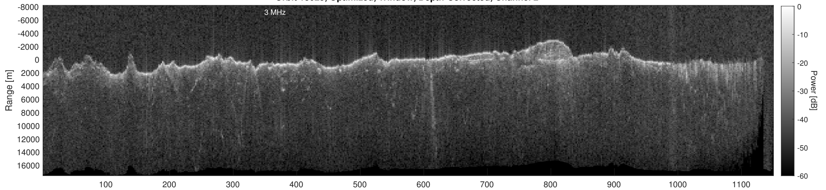
Orbit 13025, Depth-Corrected Cluttergram
