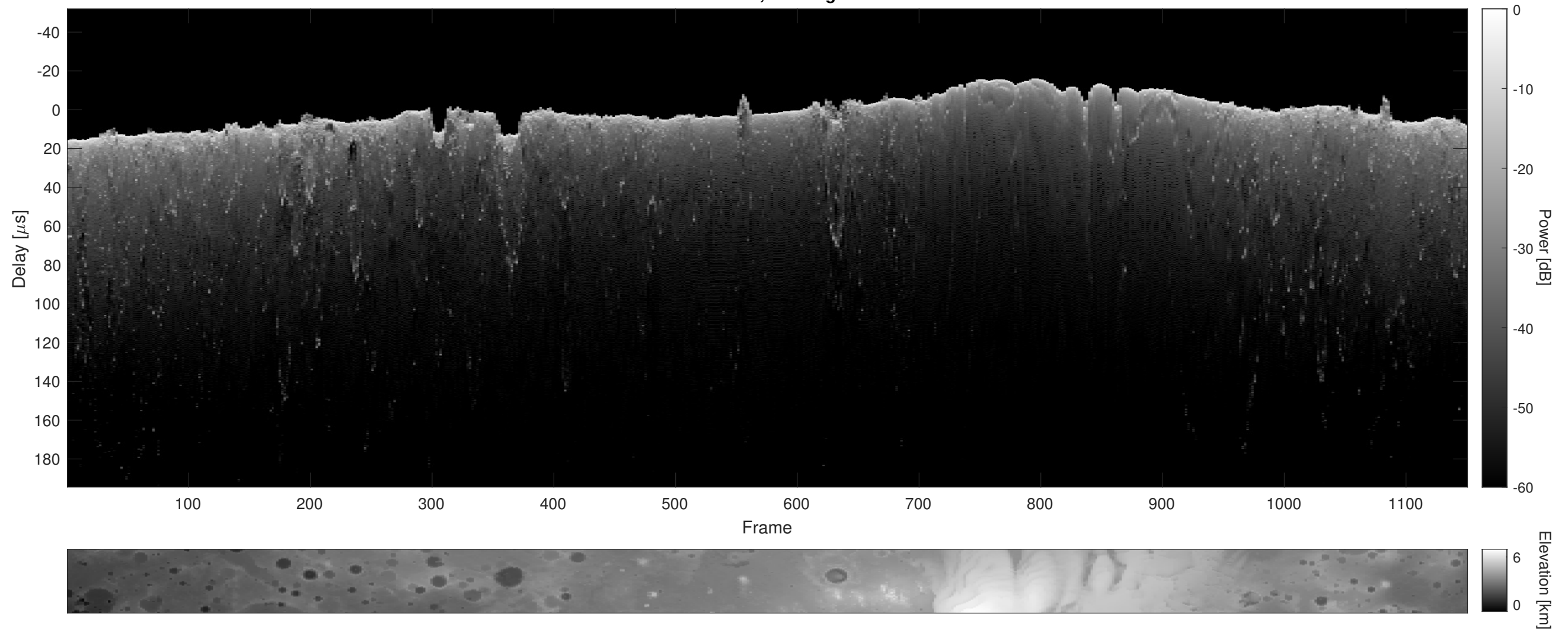
Orbit 13027, Cluttergram
