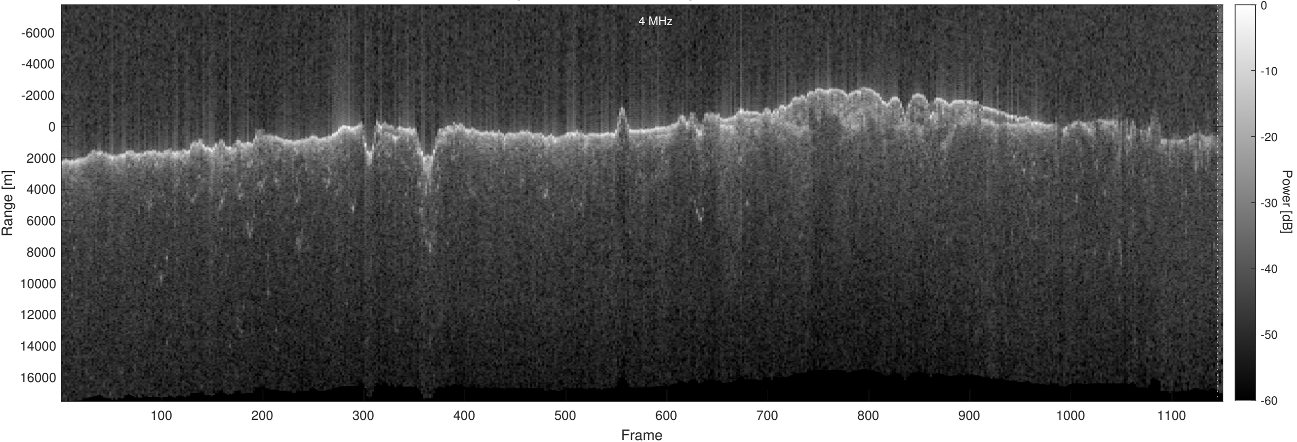
Orbit 13027, Optimized, No Window, Depth-Corrected, Channel 2
