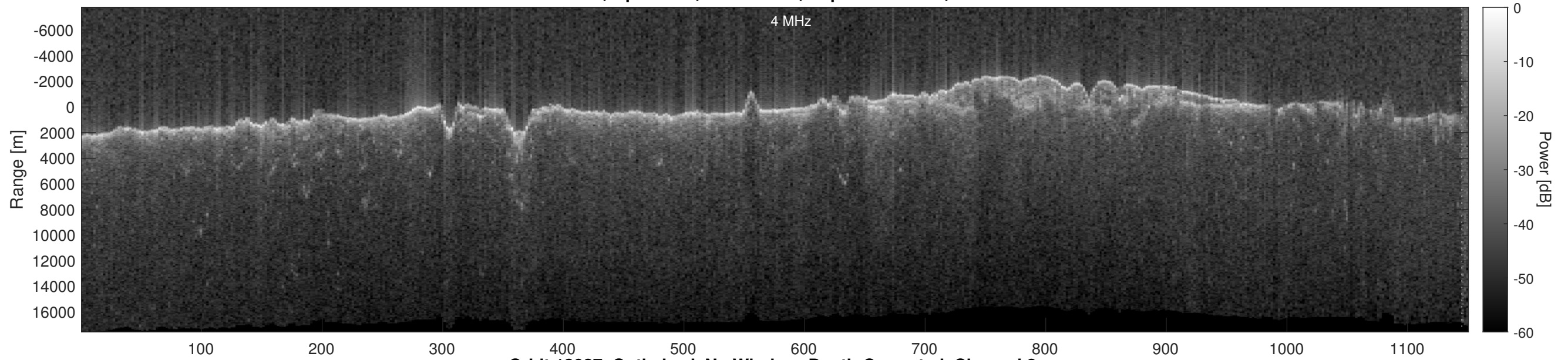
Orbit 13027, Optimized, No Window, Depth-Corrected, Channel 2
