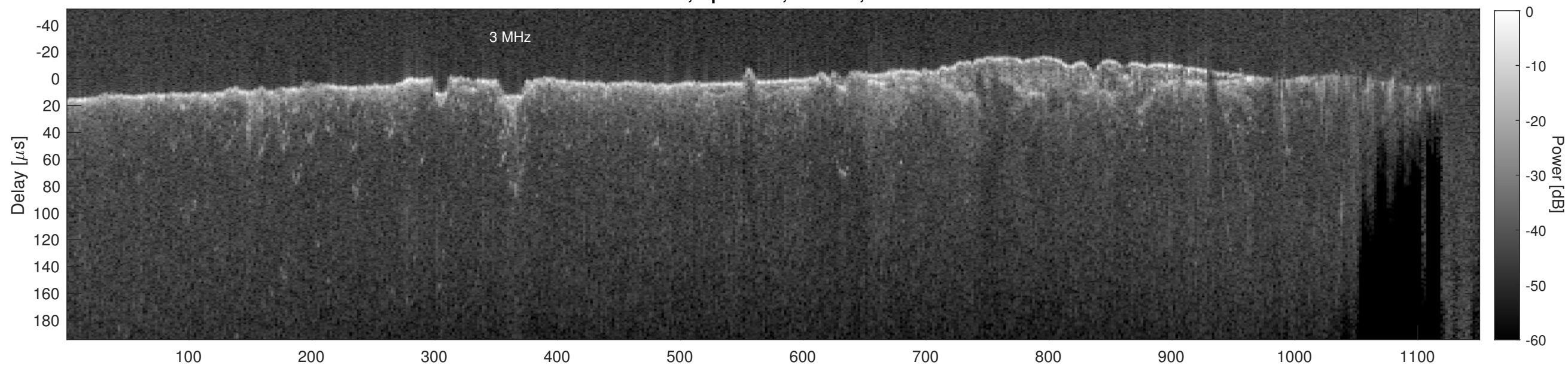
Orbit 13027, Cluttergram
