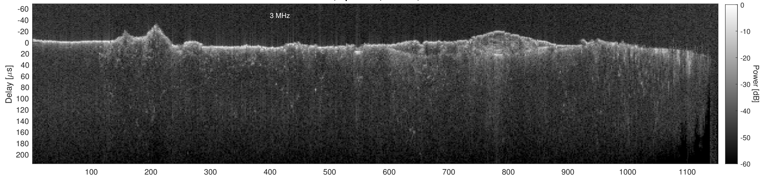
Orbit 13028, Cluttergram
