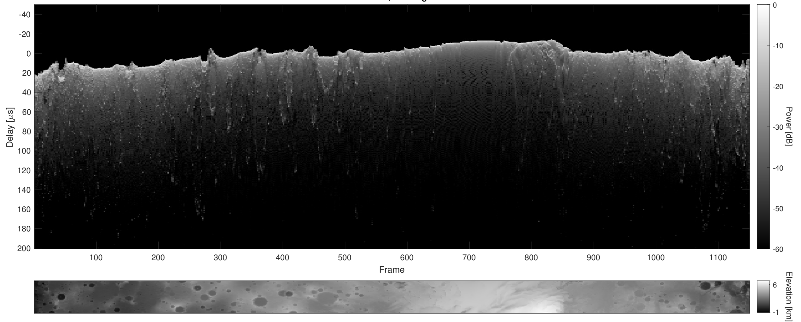
Orbit 13029, Cluttergram
