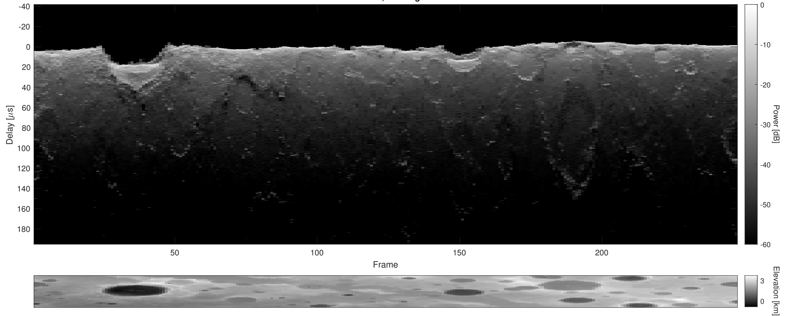
Orbit 13034, Cluttergram
