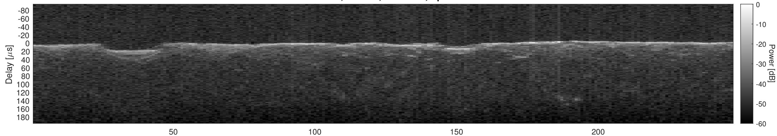
Orbit 13034, Cluttergram
