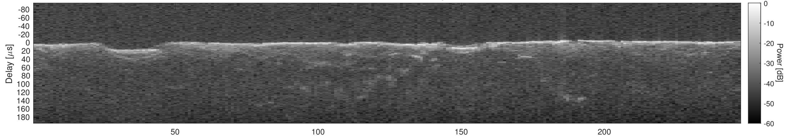
Orbit 13034, Cluttergram
