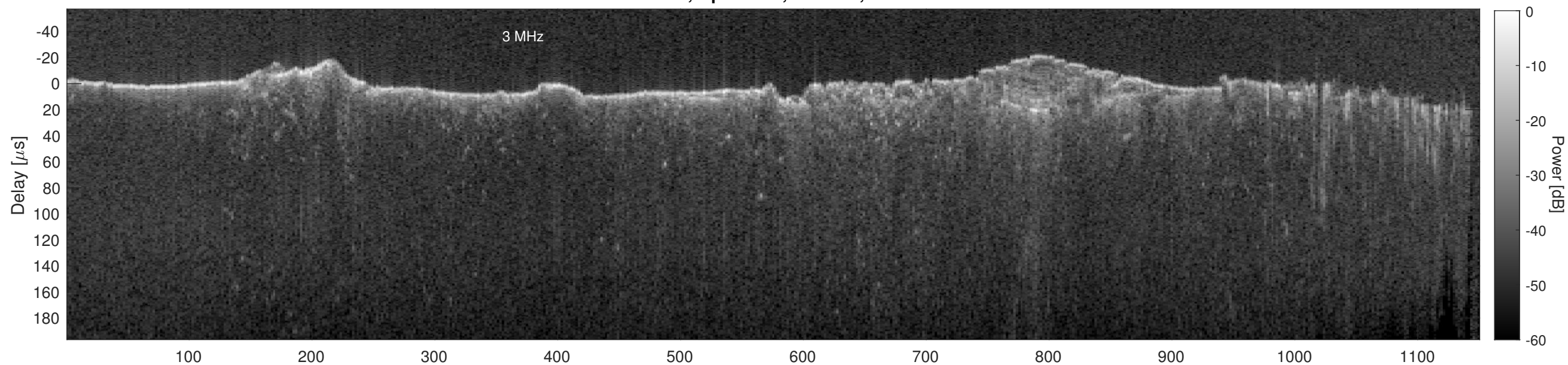
Orbit 13035, Cluttergram
