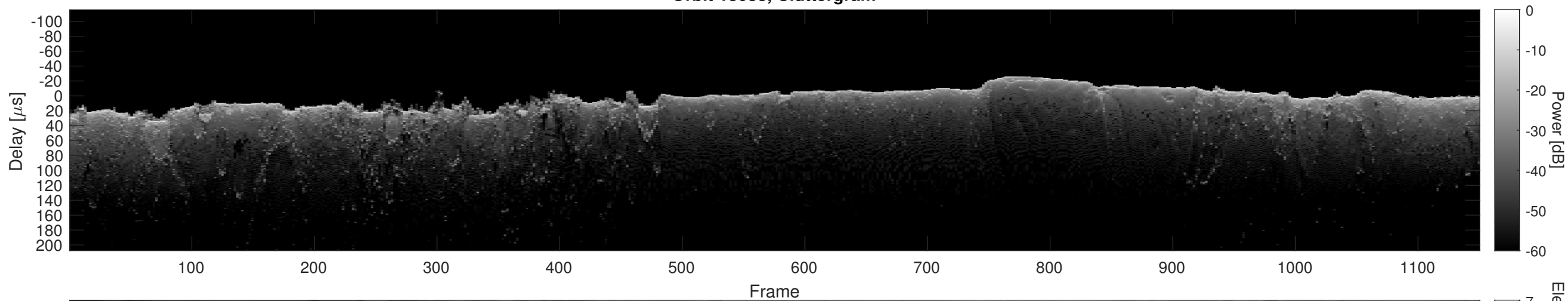
Orbit 13038, Cluttergram
