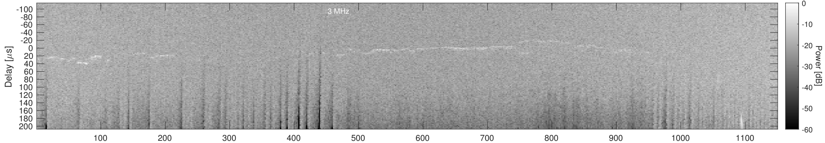
Orbit 13038, Window, Channel 2, Chapman
