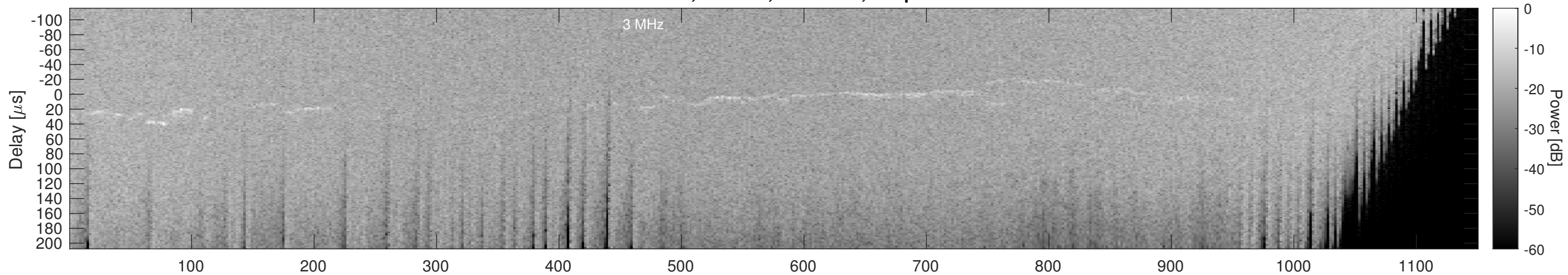
Orbit 13038, Window, Channel 2, Optimized
