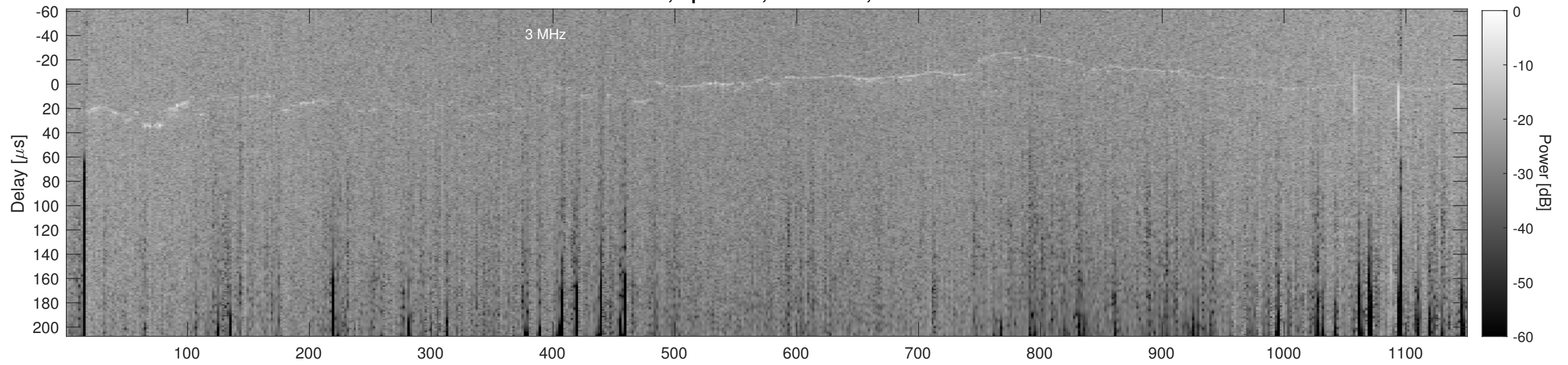
Orbit 13038, Cluttergram
