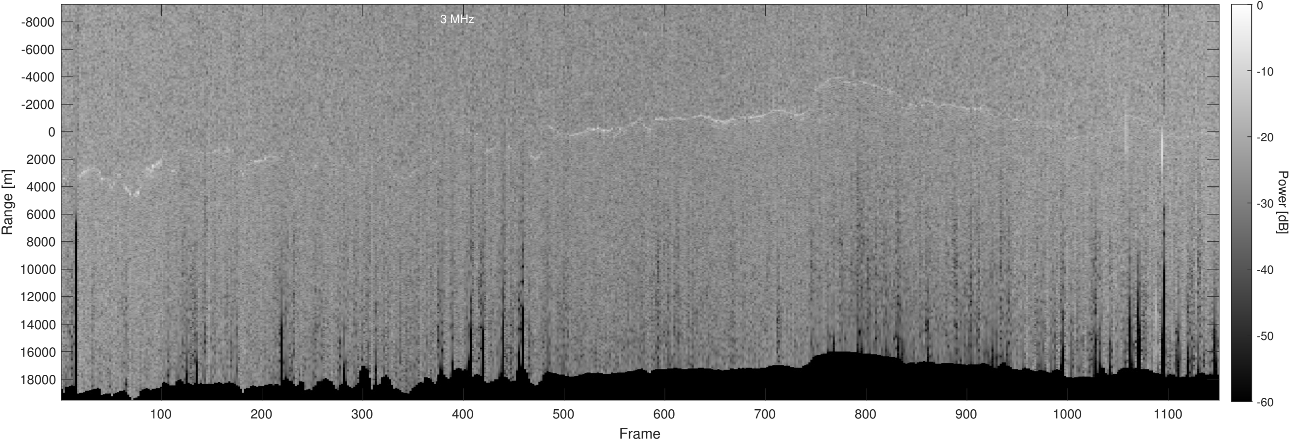
Orbit 13038, Optimized, No Window, Depth-Corrected, Channel 2
