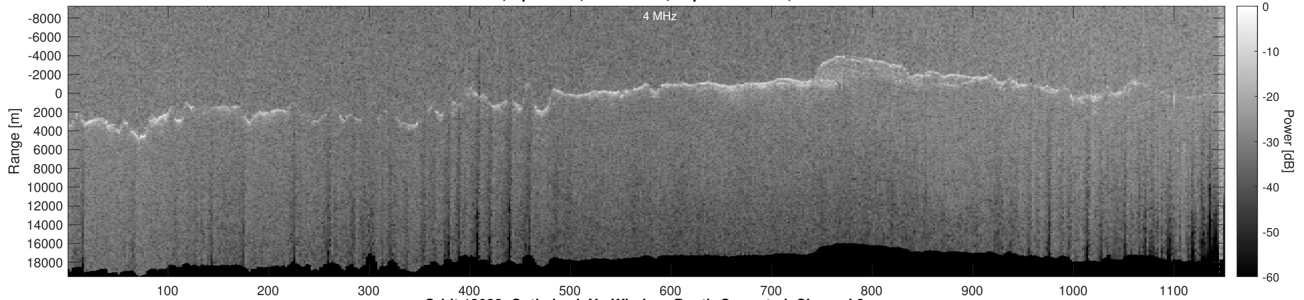
Orbit 13038, Optimized, No Window, Depth-Corrected, Channel 2
