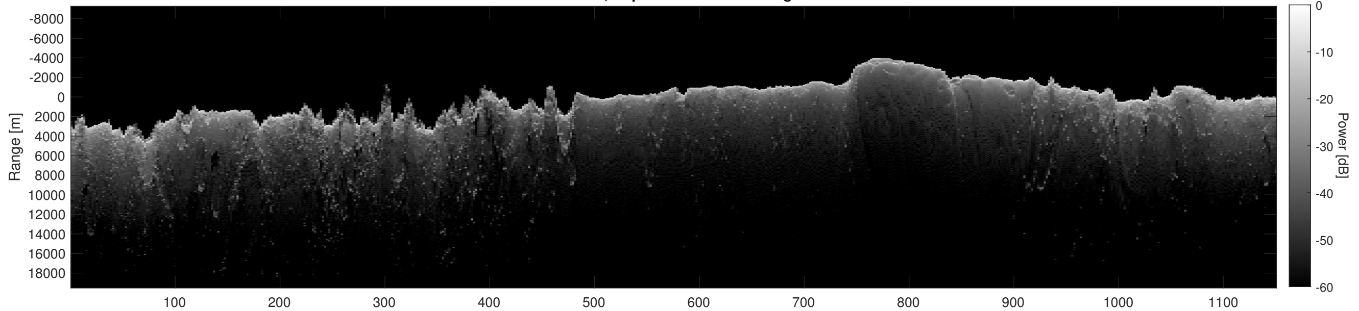
Orbit 13038, Depth-Corrected Cluttergram
