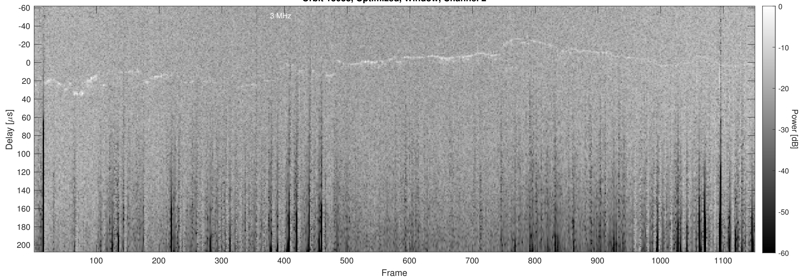
Orbit 13038, Optimized, Window, Channel 2
