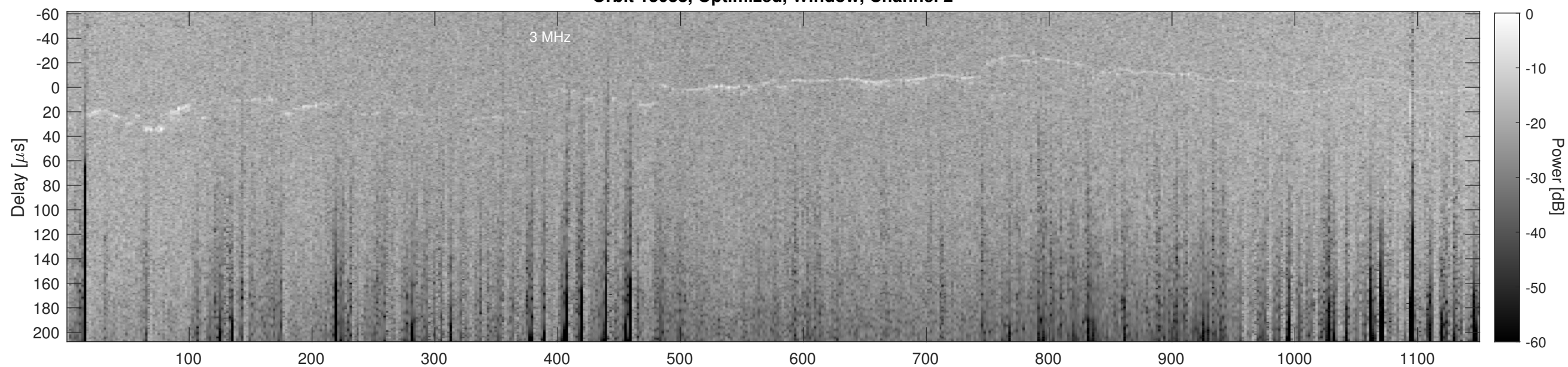
Orbit 13038, Cluttergram
