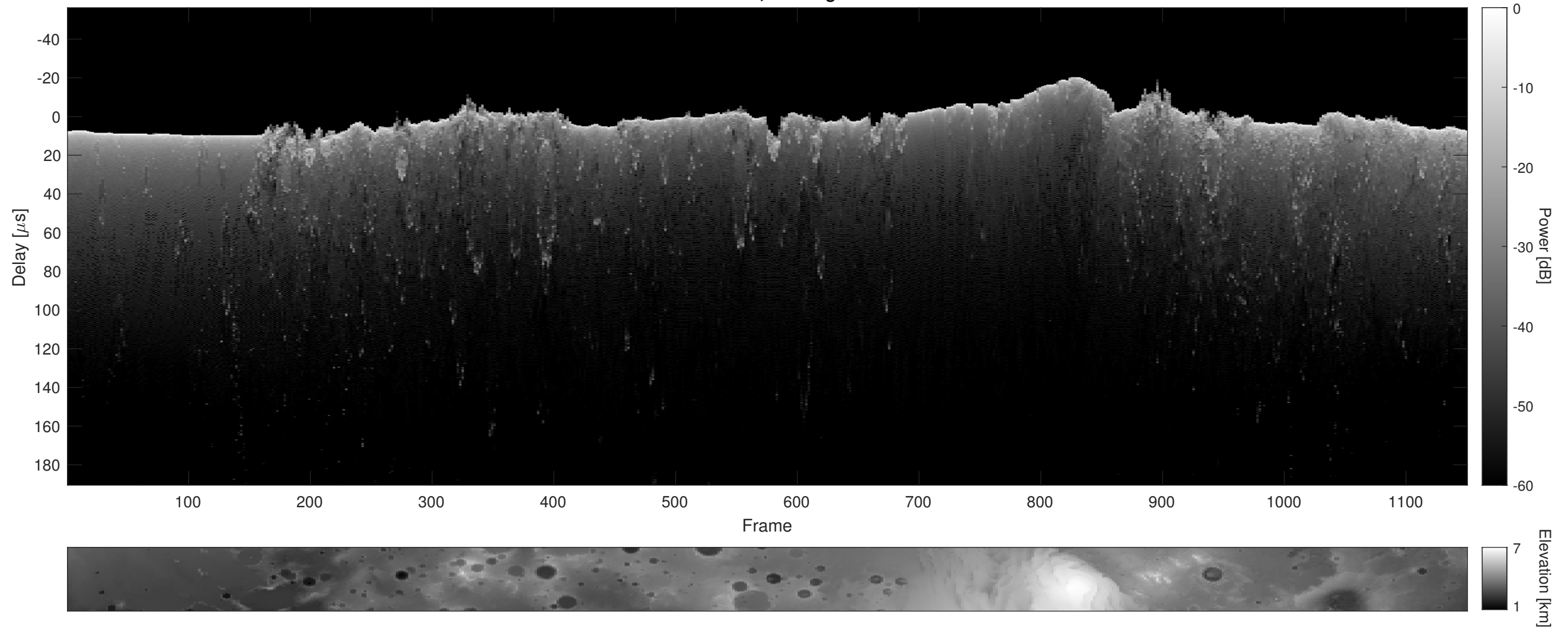
Orbit 13039, Cluttergram
