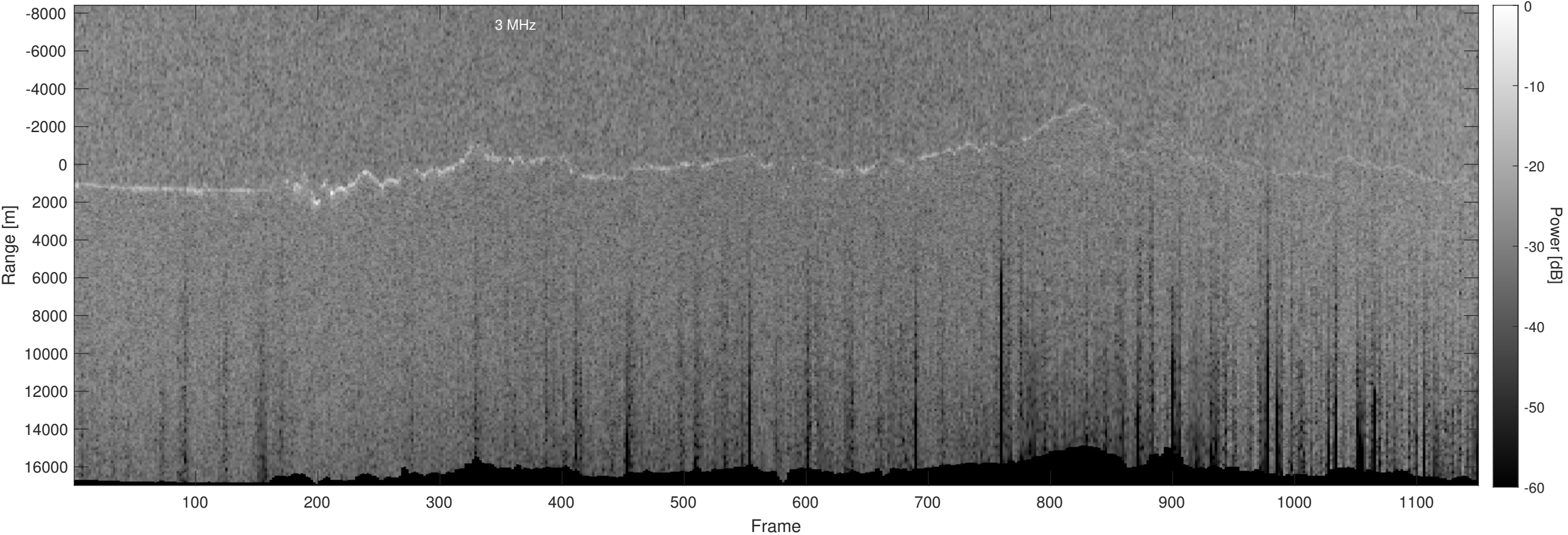
Orbit 13039, Optimized, Window, Depth-Corrected, Channel 2
