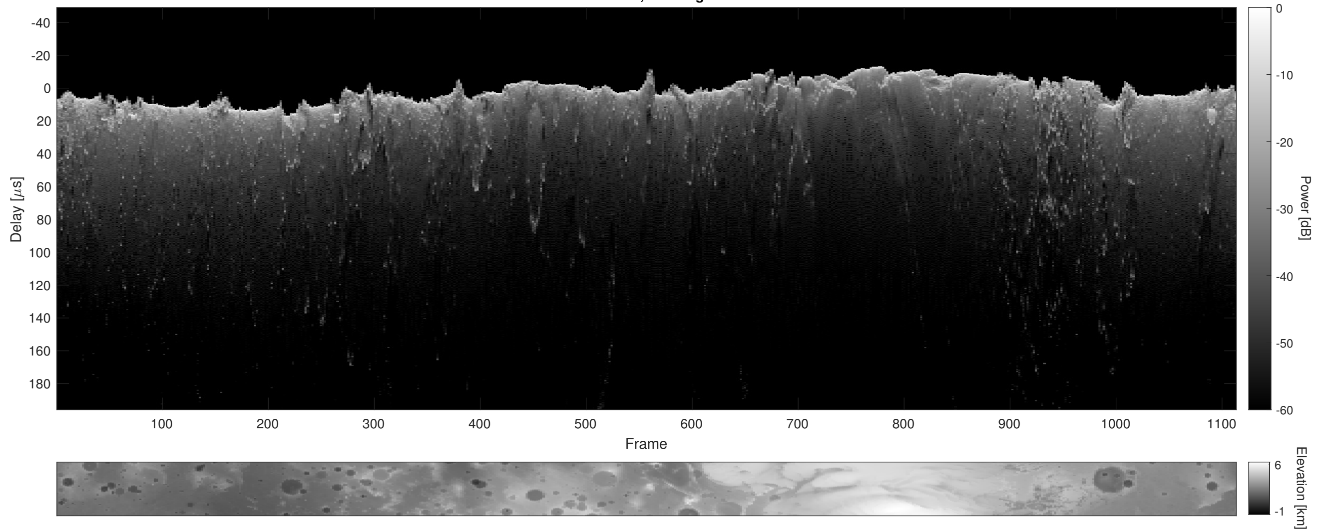
Orbit 13040, Cluttergram
