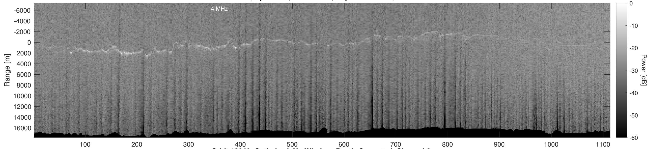
Orbit 13040, Optimized, No Window, Depth-Corrected, Channel 2
