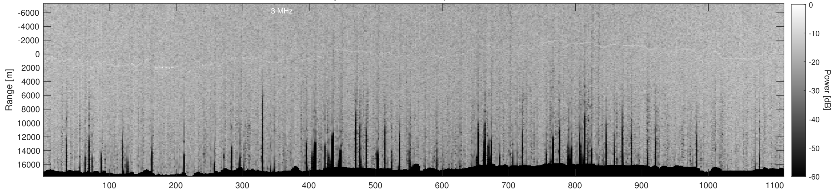
Orbit 13040, Depth-Corrected Cluttergram
