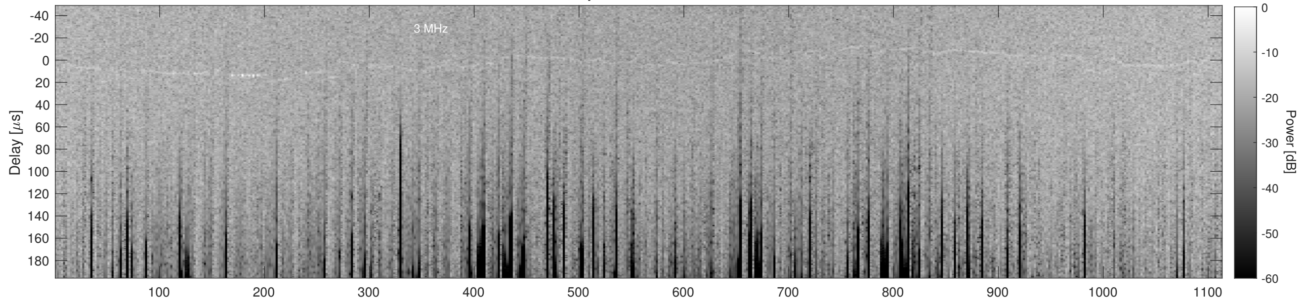
Orbit 13040, Cluttergram
