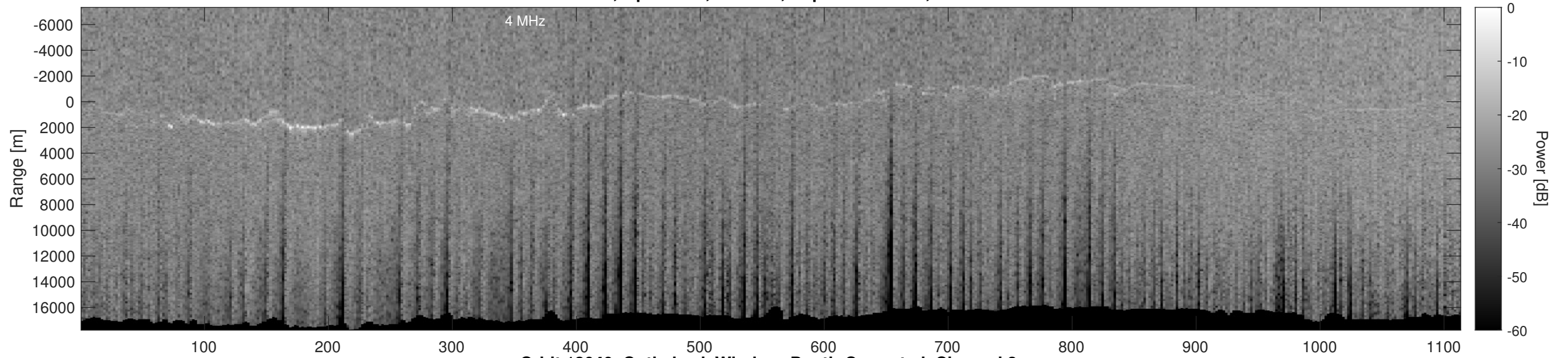
Orbit 13040, Optimized, Window, Depth-Corrected, Channel 2
