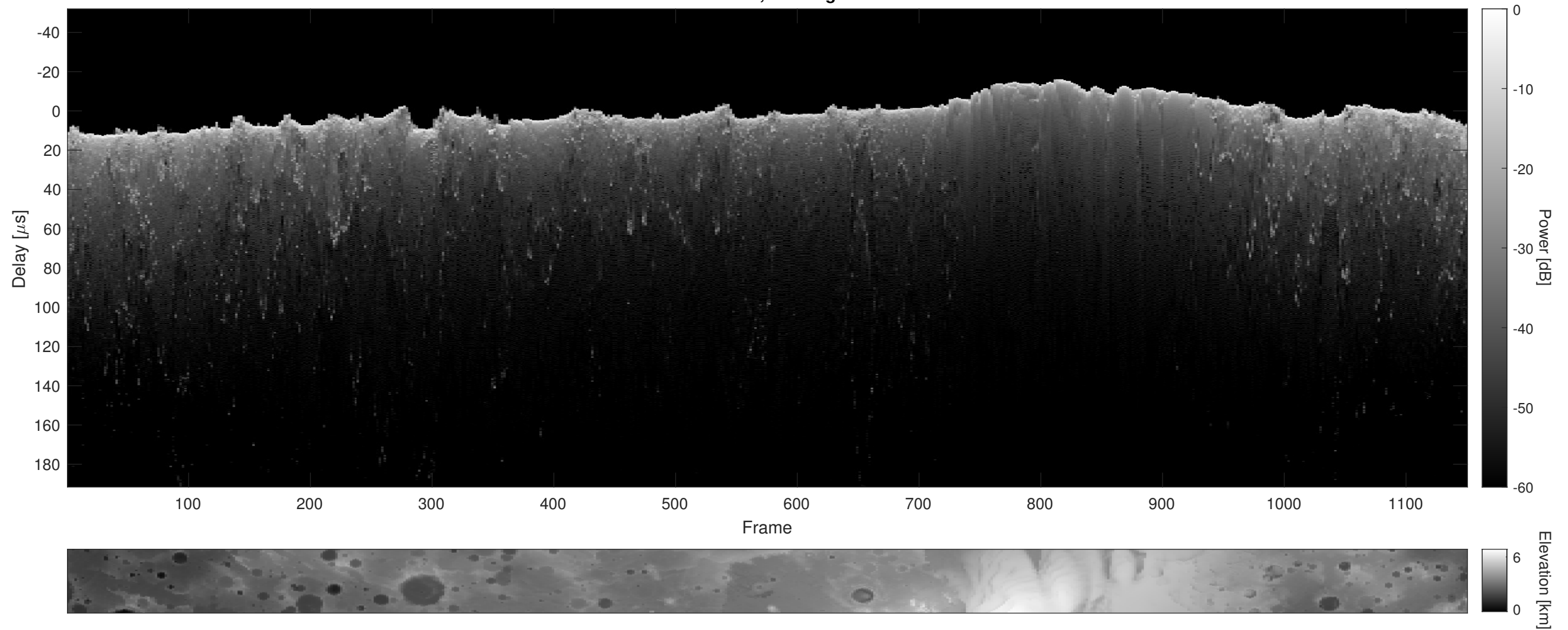
Orbit 13041, Cluttergram
