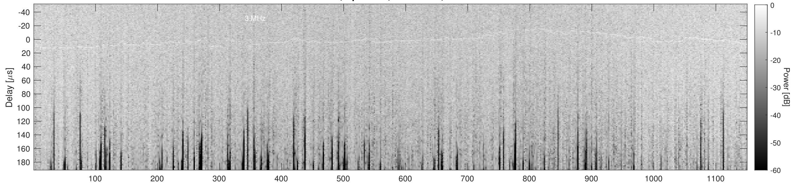
Orbit 13041, Cluttergram
