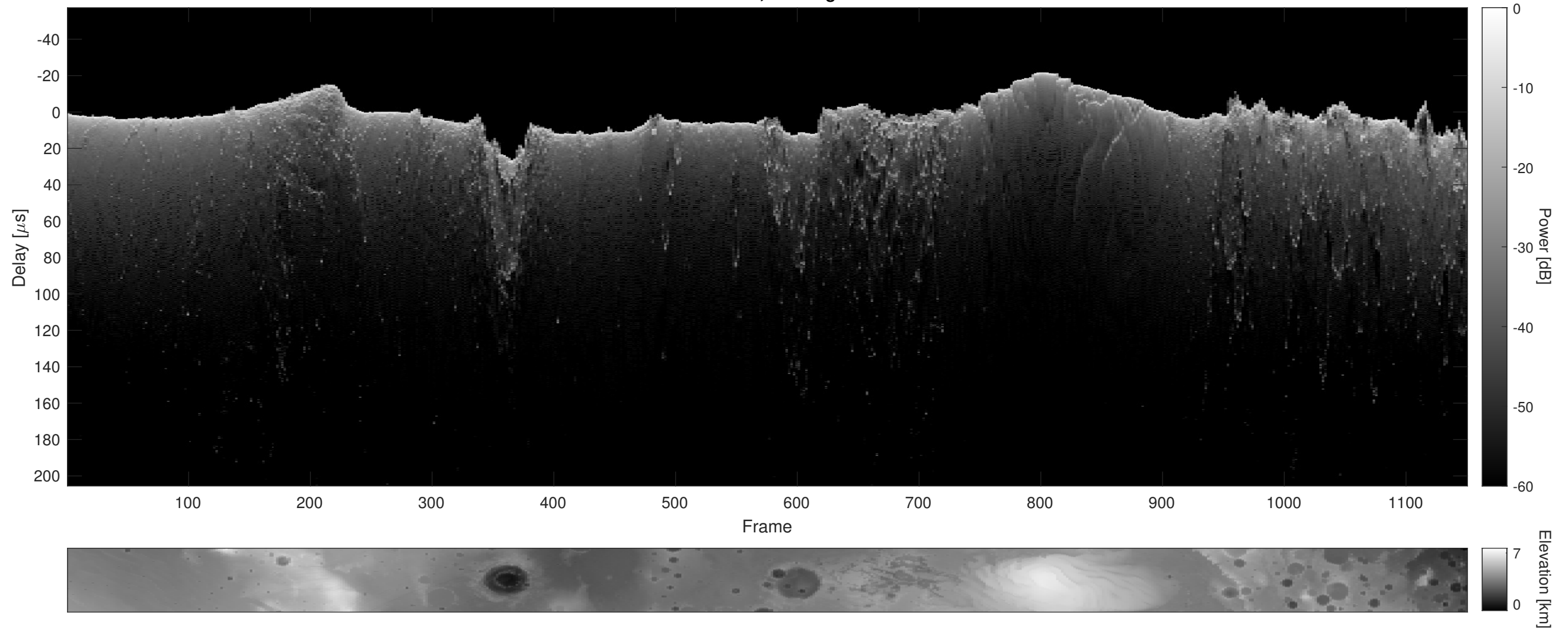
Orbit 13042, Cluttergram
