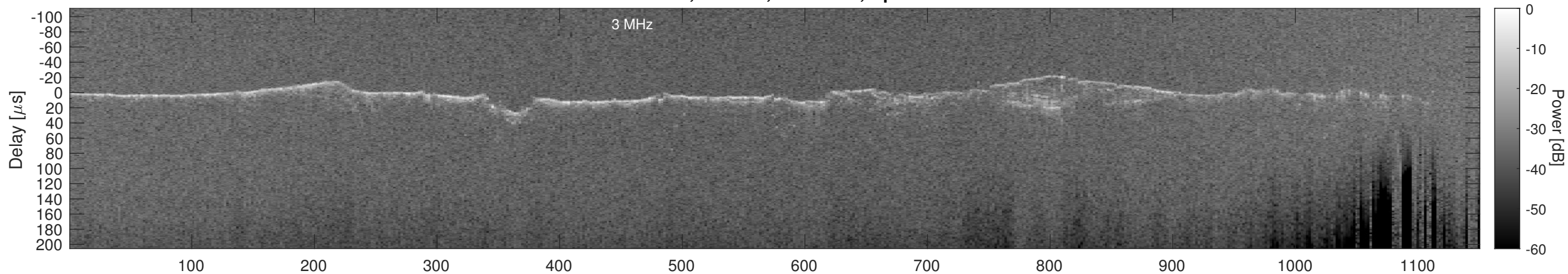
Orbit 13042, Cluttergram
