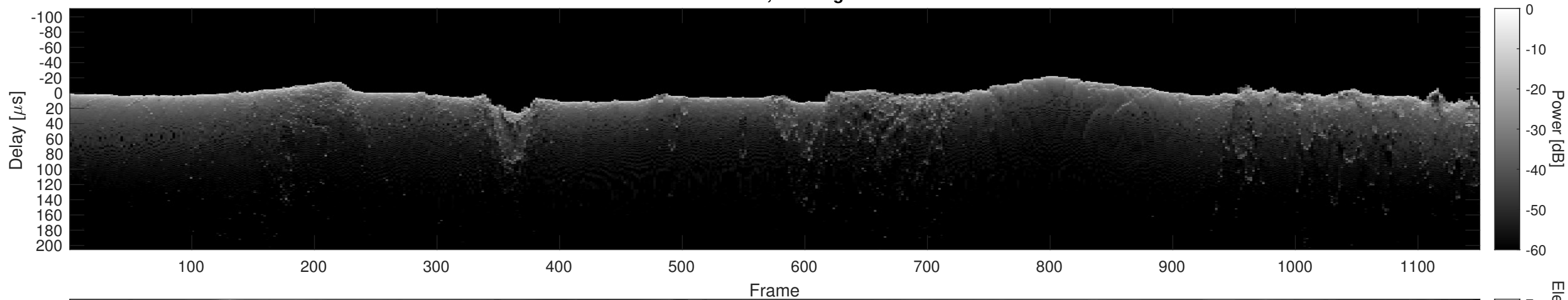
Orbit 13042, Cluttergram
