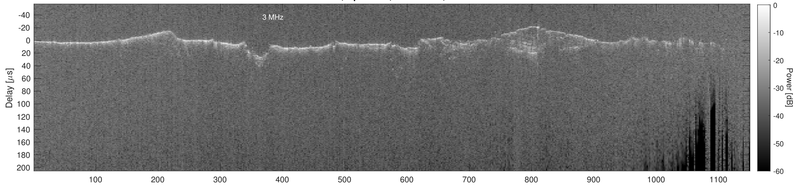
Orbit 13042, Cluttergram
