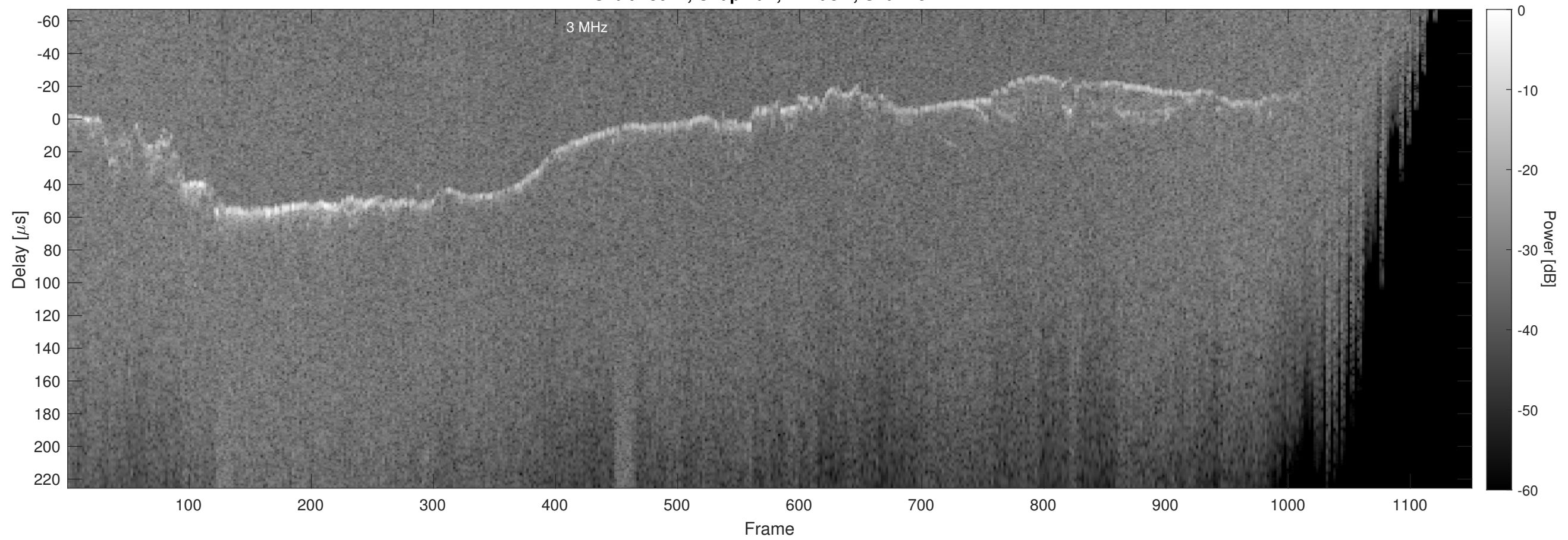
Orbit 13044, Chapman, Window, Channel 2
