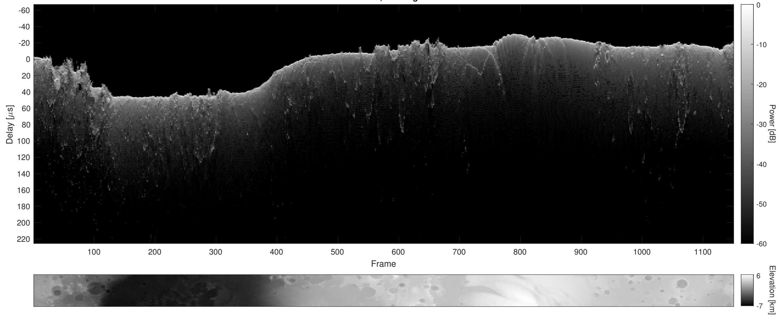
Orbit 13044, Cluttergram
