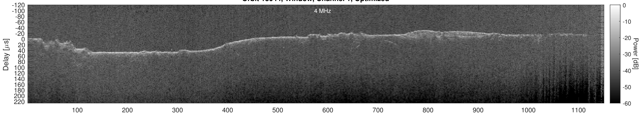
Orbit 13044, Cluttergram
