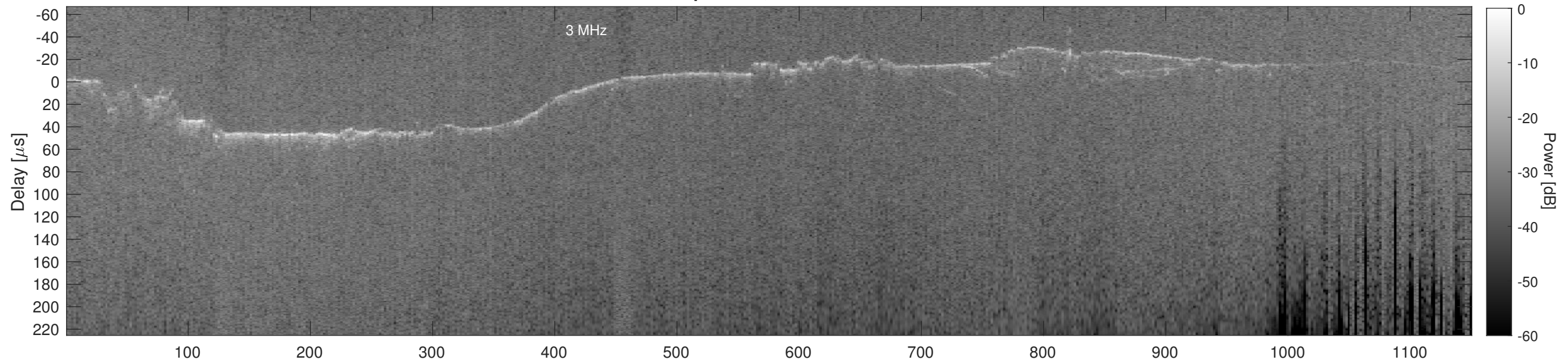
Orbit 13044, Cluttergram
