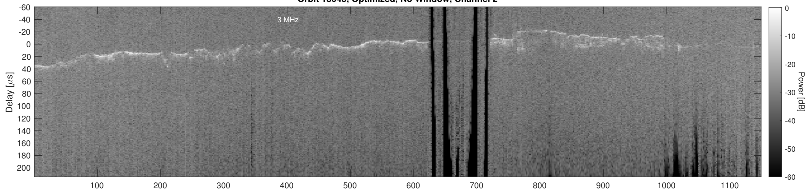
Orbit 13045, Cluttergram
