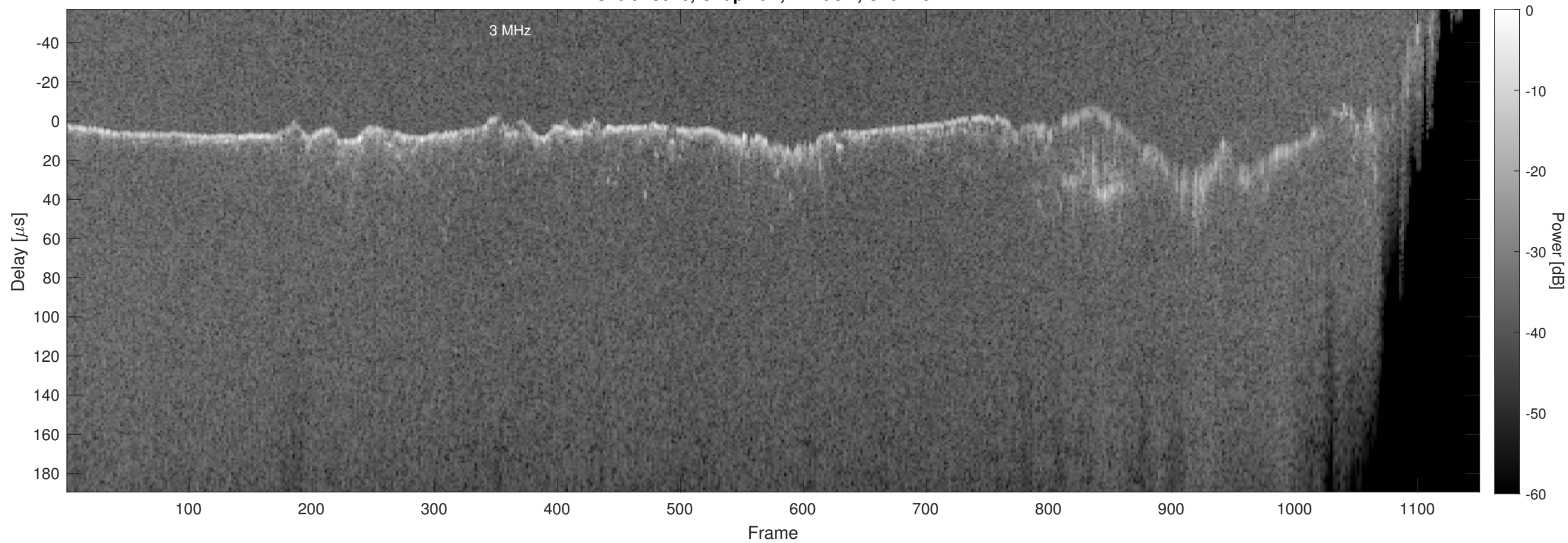
Orbit 13046, Chapman, Window, Channel 2
