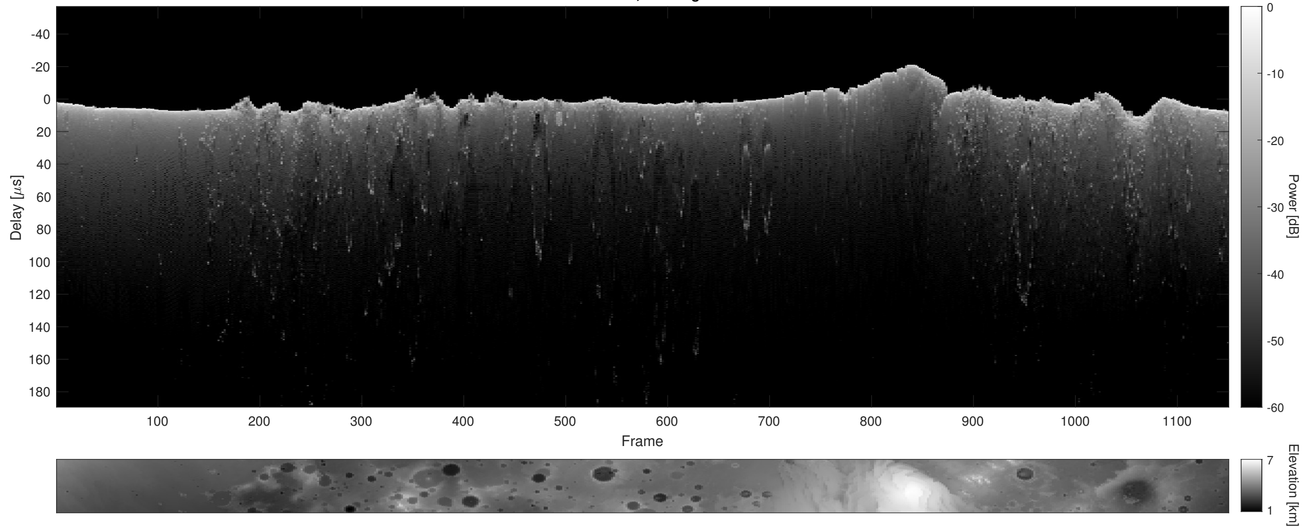
Orbit 13046, Cluttergram
