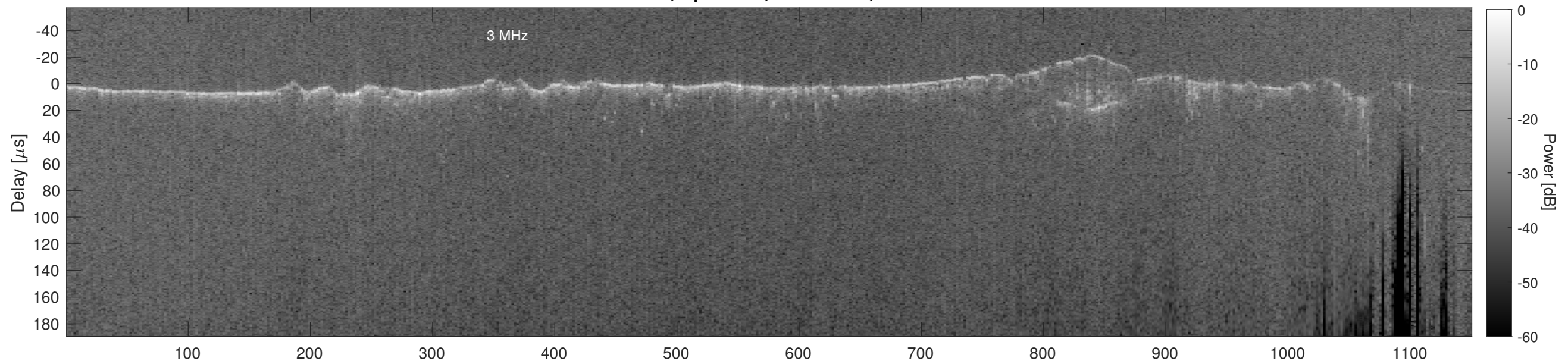
Orbit 13046, Cluttergram
