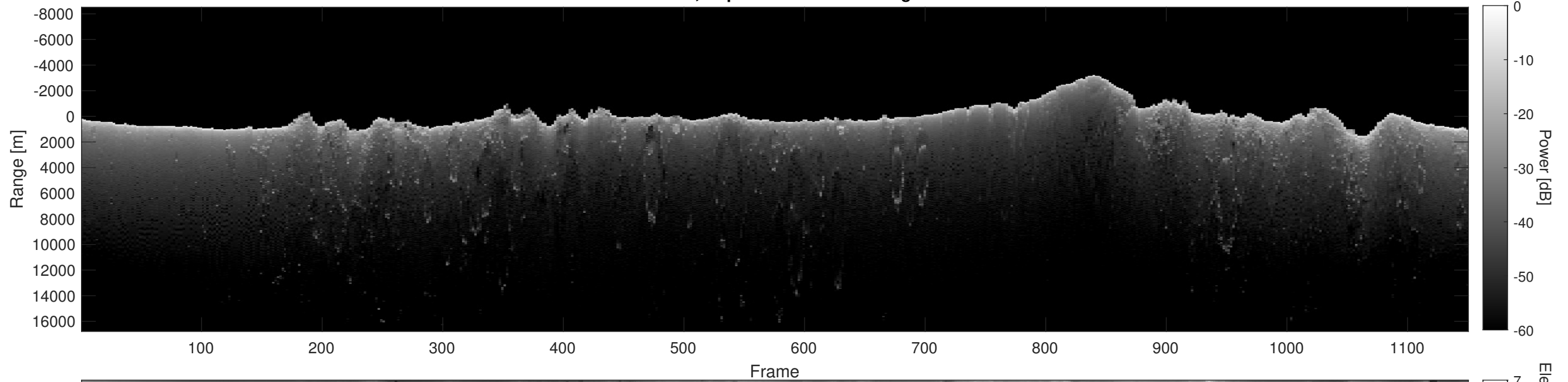
Orbit 13046, Depth-Corrected Cluttergram
