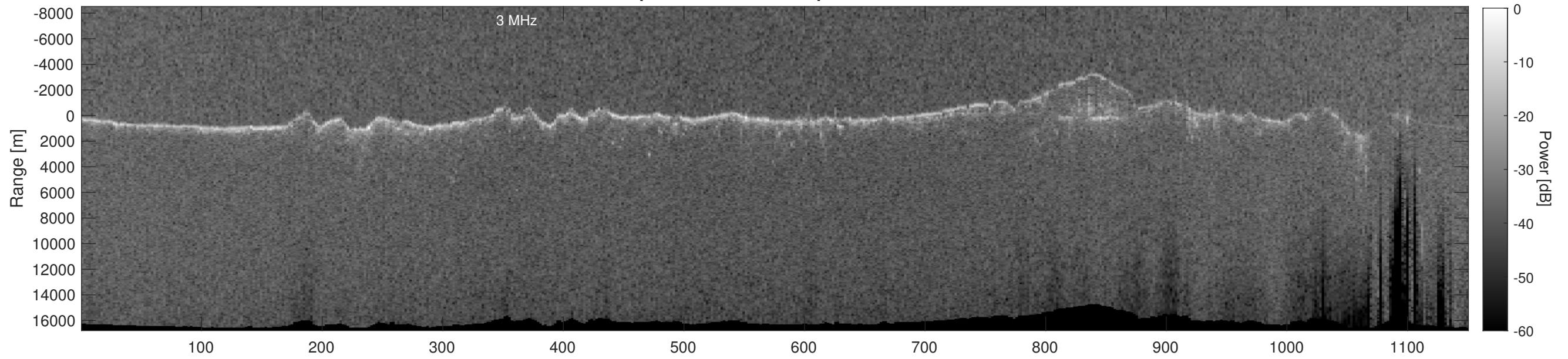
Orbit 13046, Depth-Corrected Cluttergram
