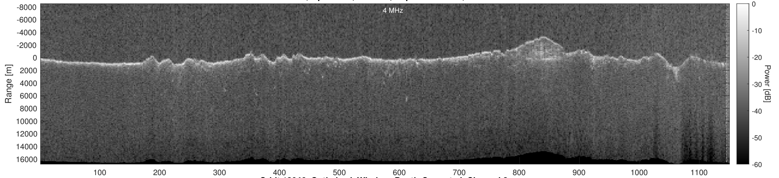
Orbit 13046, Optimized, Window, Depth-Corrected, Channel 2
