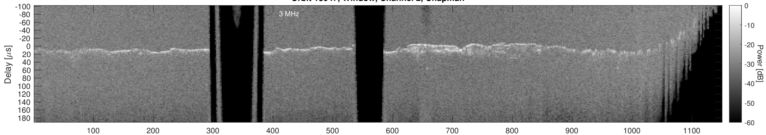
Orbit 13047, Window, Channel 2, Optimized
