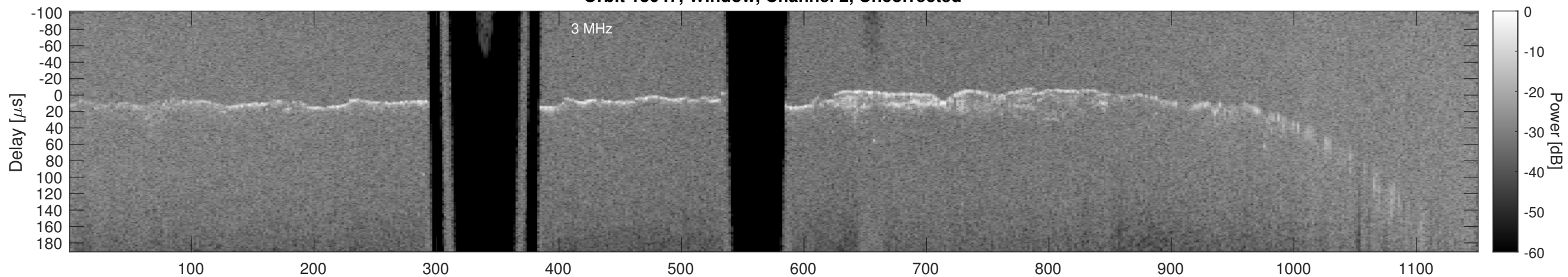
Orbit 13047, Window, Channel 2, Chapman
