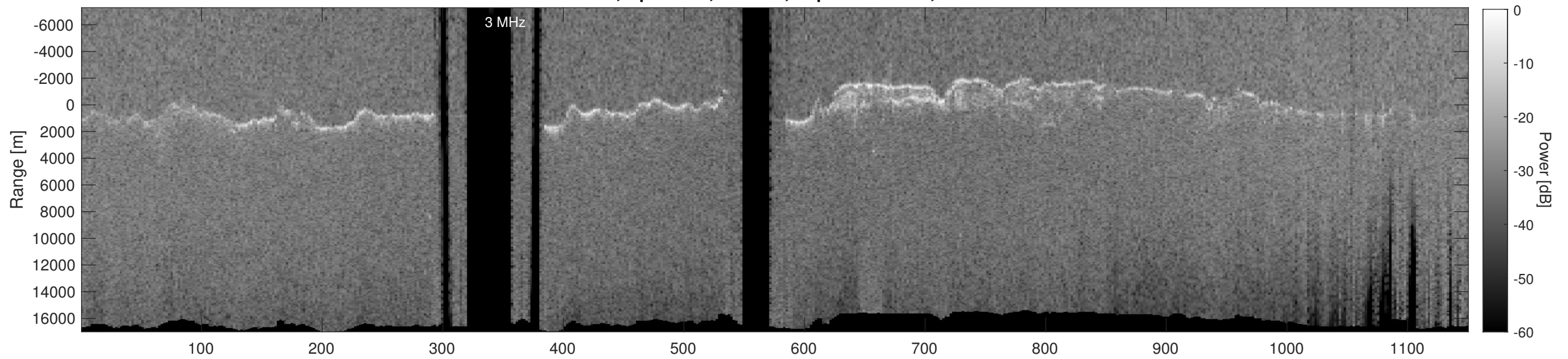
Orbit 13047, Depth-Corrected Cluttergram
