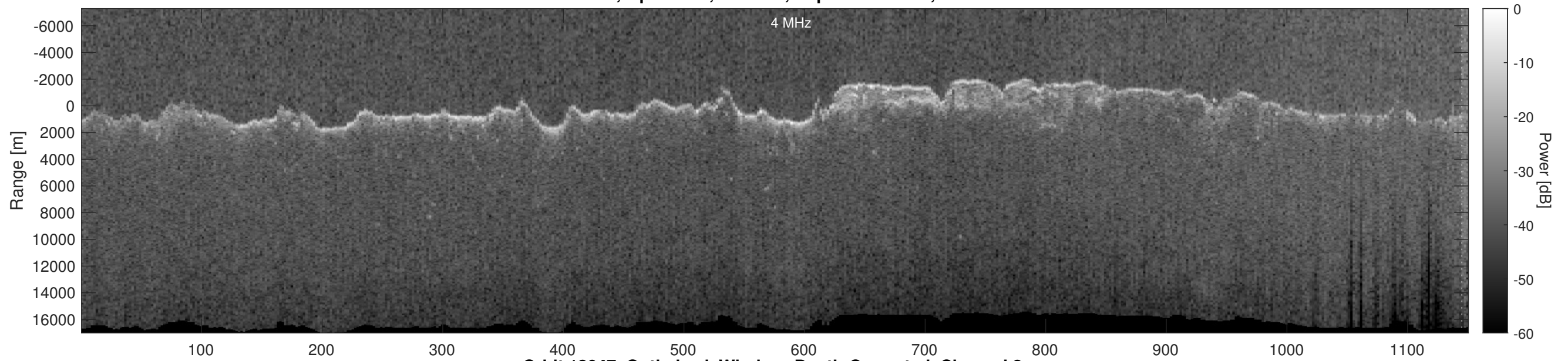
Orbit 13047, Optimized, Window, Depth-Corrected, Channel 2
