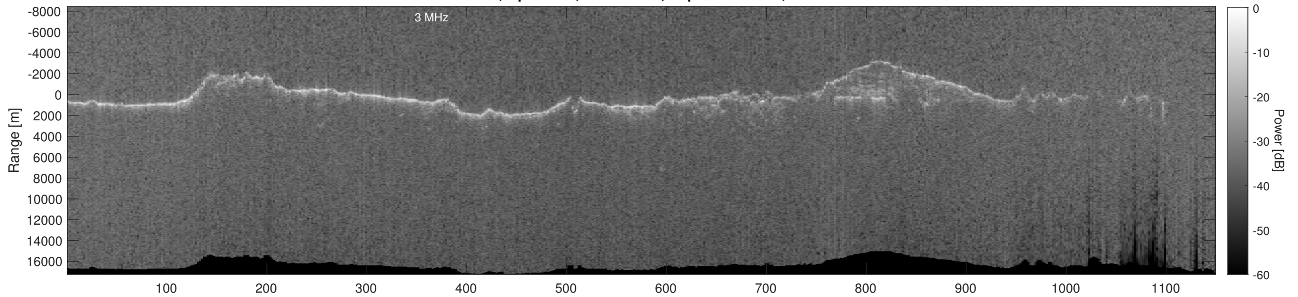
Orbit 13049, Depth-Corrected Cluttergram
